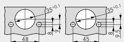
Combination drilling pattern for Impresso
